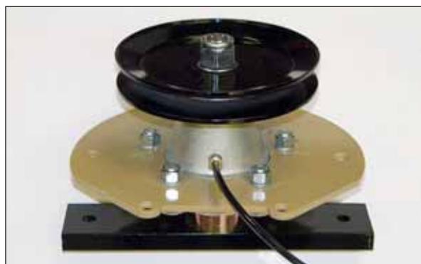
The commercial duty 1 3/8" blade spindle features a cast iron housing, additional steel plate support, a 3/4" thick blade support bar and a remote greasing line.
