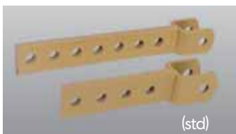
Some tractor and tire combinations do not allow enough room for the mower hook-up. Longer lower hitch clevises are available to easily correct this situation.
